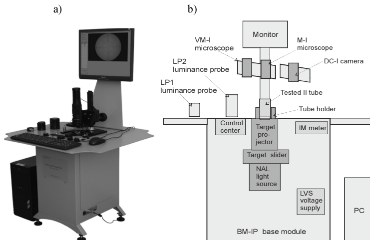
Fig. 1. The ITS-I test station: a) a photo; b) a block diagram.
