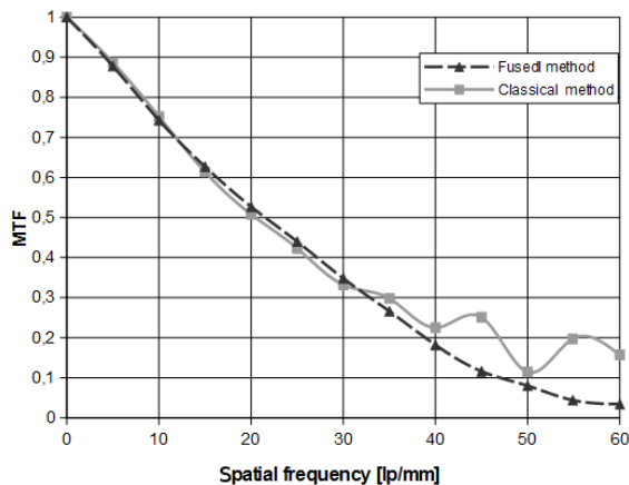
Fig. 6. The MTF measurement results of an exemplary IIT obtained using two measurement methods.
