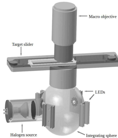
Fig. 5. A 3D drawing of the NAL light source.
