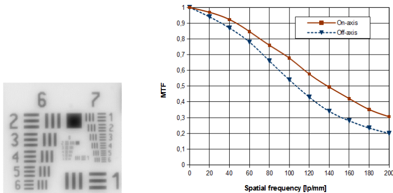
Fig. 4. The test results of the macro objective: the image of USAF 1951 target projected by the objective (left), the MTF measurement results (right).
