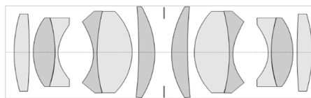
Fig. 3. An optical diagram of the optical macro objective used as the image projector in the ITS-IP test station.
